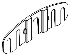
9 Spacer A hebt die Front Spacer A raises the front
